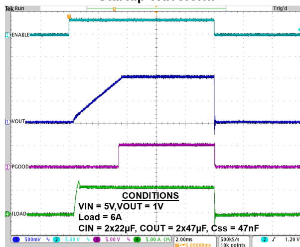
Startup Waveform
