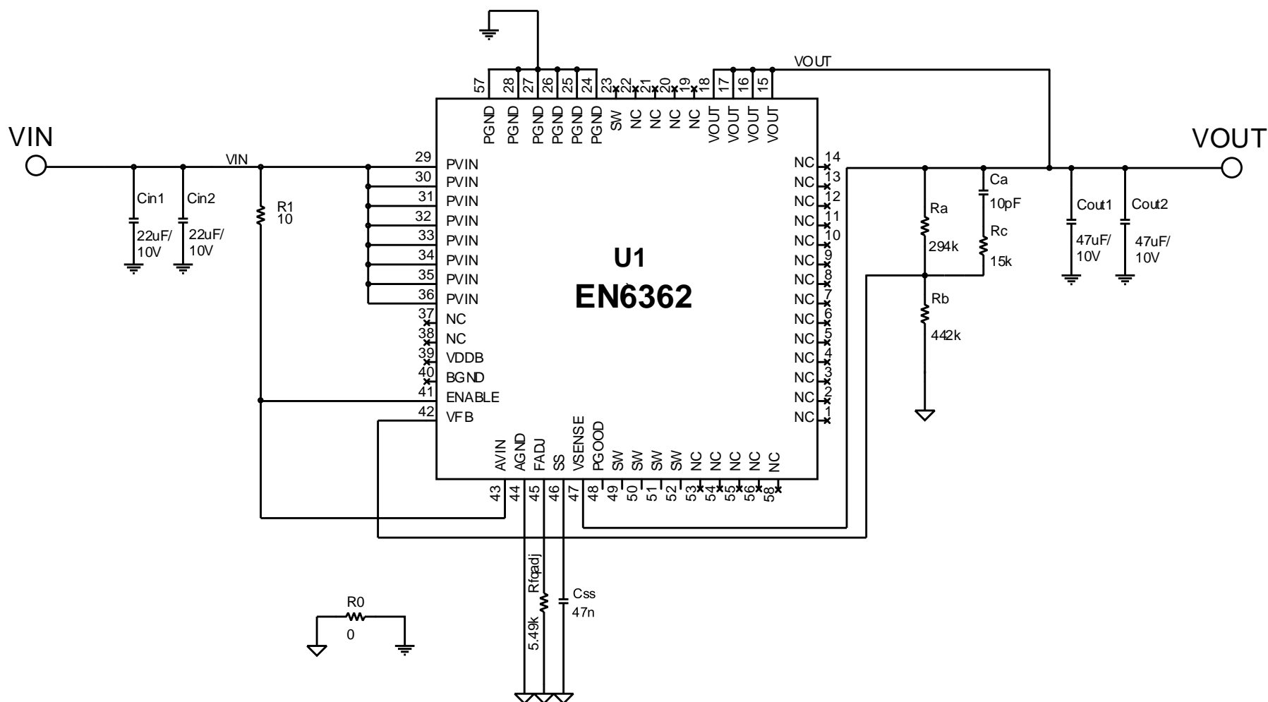
Figure 7: Application Schematic
