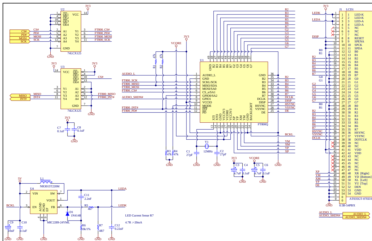
Figure 4-1 - VM800C35 ( 3.5" Version)
