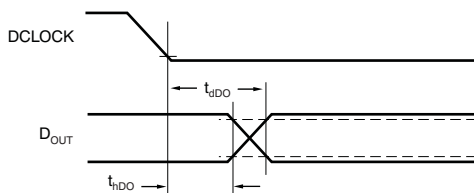
Voltage Waveforms for D_{\text{OUT}} Delay Times, t_{\text{dDO}}
