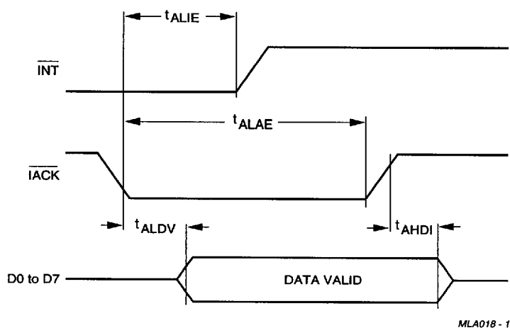
Fig.19 Interrupt timing (80XX mode).
