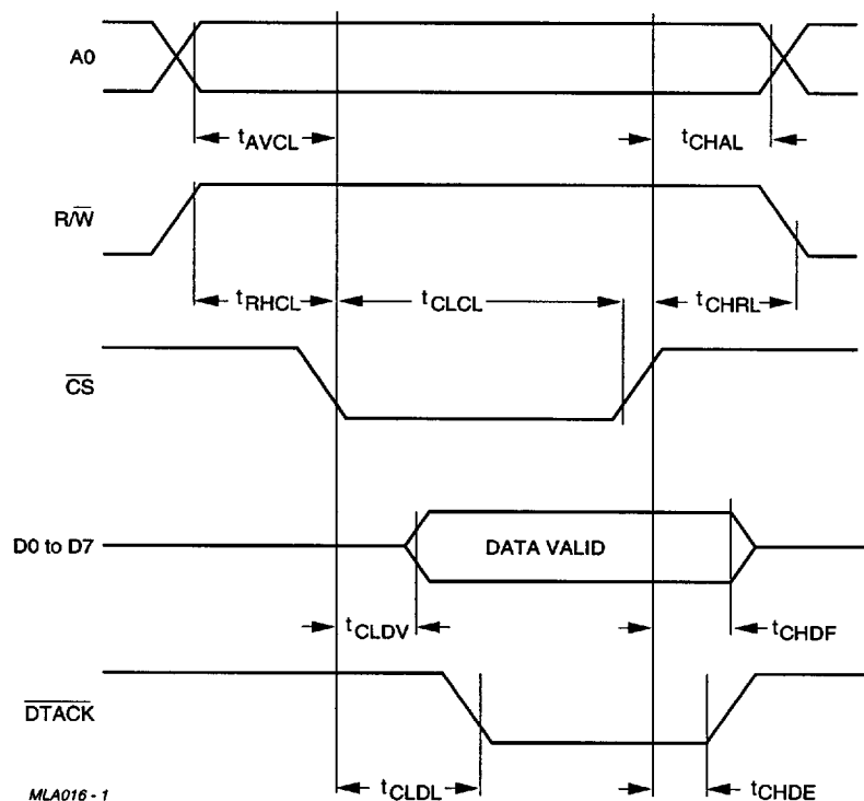
Fig.18 Bus timing (68000 mode); read cycle.
