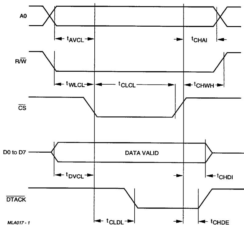
Fig.17 Bus timing (68000 mode); write cycle.
