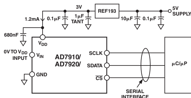
Figure 7. REF193 as Power Supply
