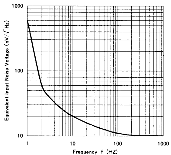
NJM14558 Equivalent Input Noise Voltage vs. Frequency
