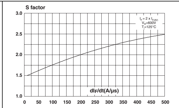
Figure 8. Softness factor versus dl_F/dt (typical values)
