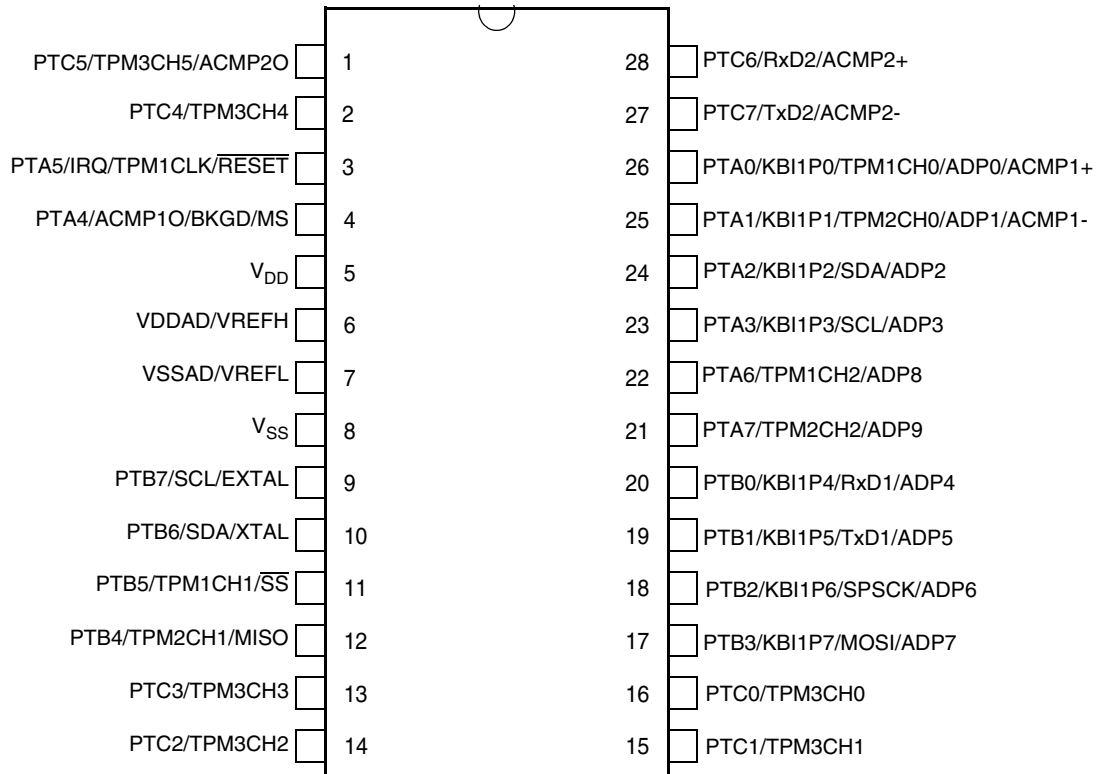
Figure 2-5. 28-pin SOIC
