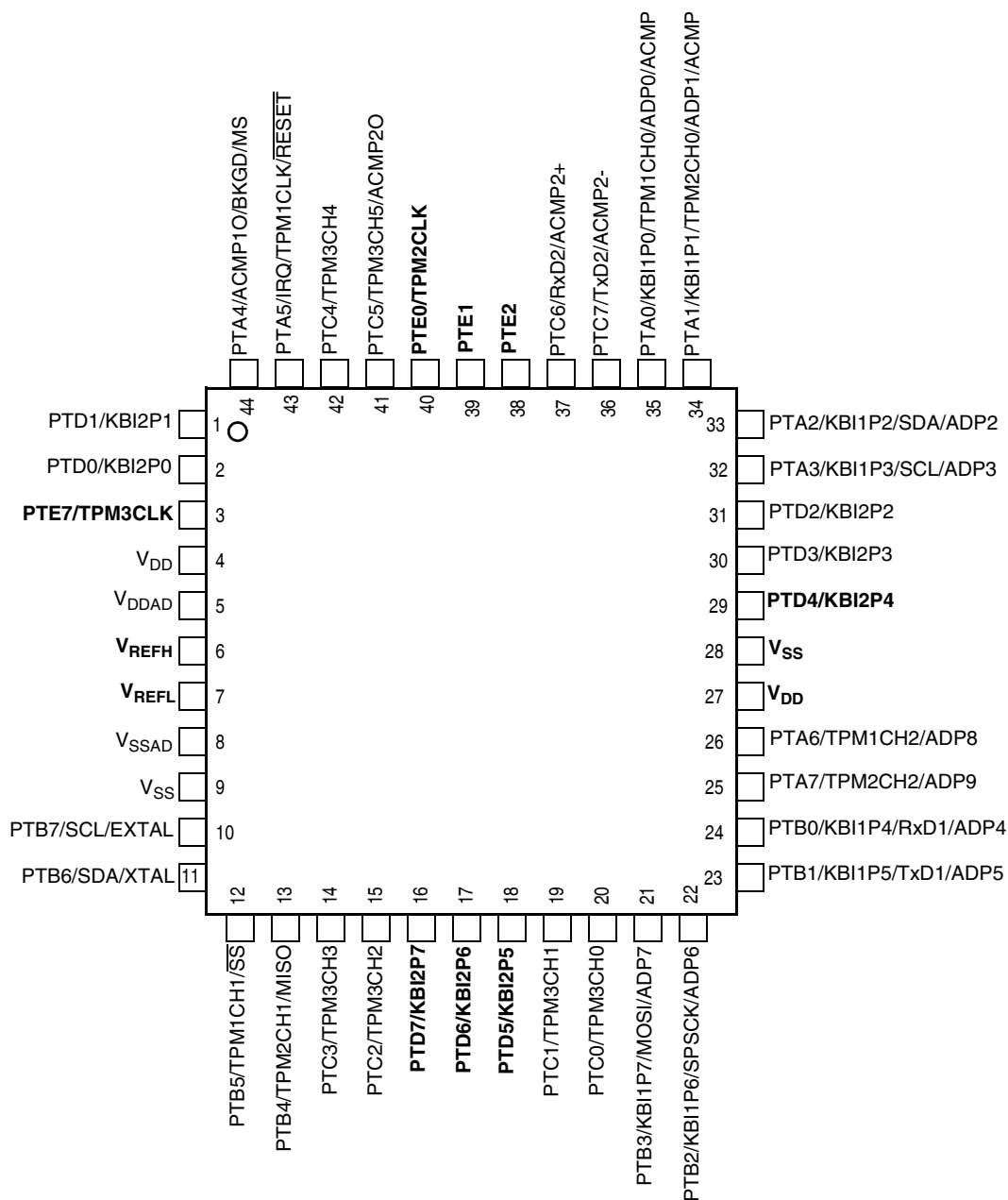
Figure 2-3. 44-pin LQFP
