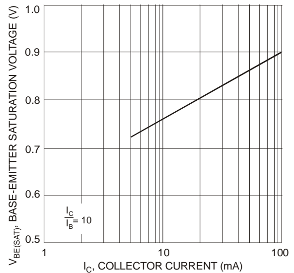
Fig. 4 Typical Base-Emitter Saturation Voltage vs. Collector Current (PNP-4126)
