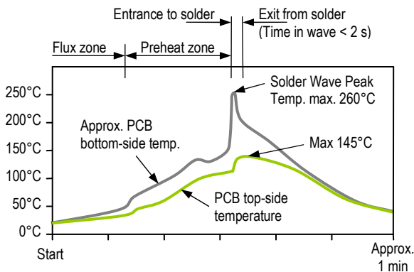
Figure 6: Suitable wave soldering profile.
