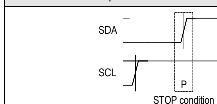
I 2 C Transmission Stop Condition
