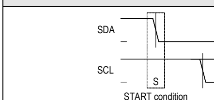
I 2 C Transmission Start Condition
