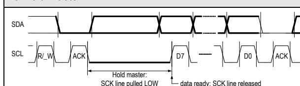
I 2 C Hold Master
