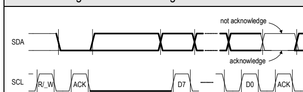
I 2 C Acknowledge / Not Acknowledge
