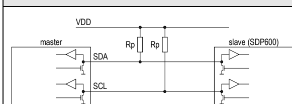
I 2 C Transmission Start Condition
