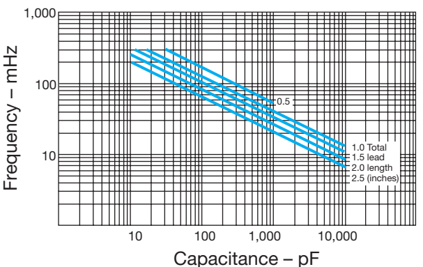
Resonant Frequency vs. Capacitance Axial
