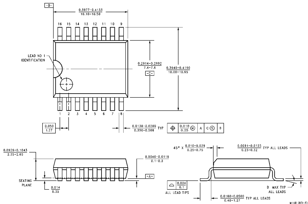
Figure 10. 16-Lead Small Outline Integrated Circuit (SOIC), JEDEC MS-013, 0.300" Wide Package Number M16B
