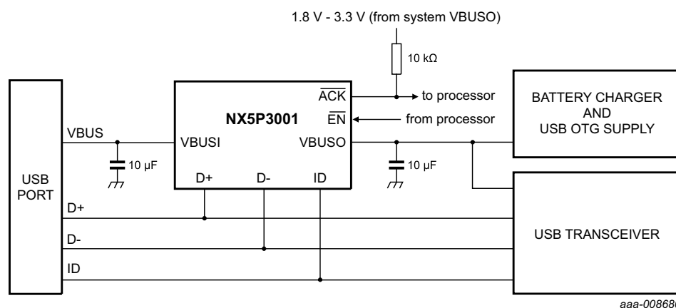
Fig 5. NX5P3001 application diagram
