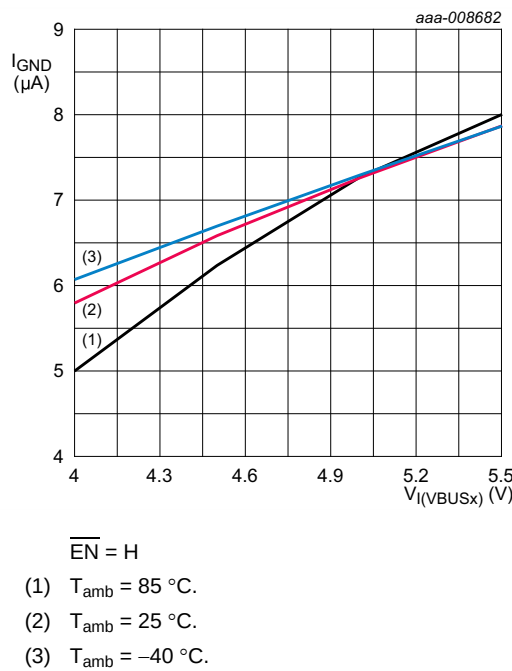
Fig 8. Ground current versus input voltage on pin VBUSI or VBUSO
