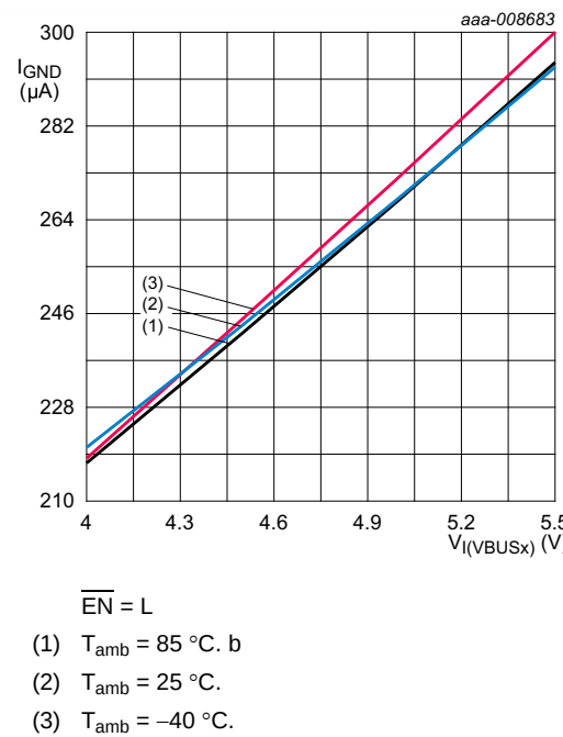
Fig 9. Ground current versus input voltage on pin VBUSI or VBUSO
