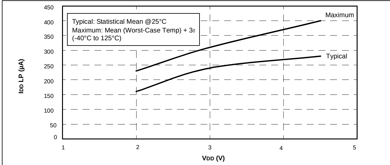
FIGURE 17-18: PIC12HV609/615 I_{DD\ LP} (32 kHz) vs. V_{DD}
