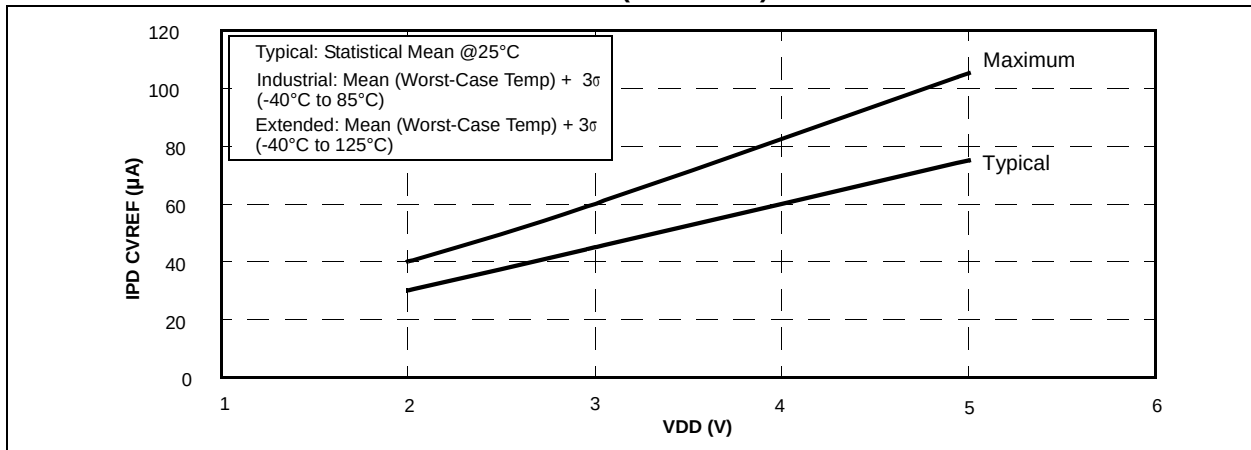
FIGURE 17-15: PIC12F609/615/617 I PD CVREF (HI RANGE) vs. V DD
