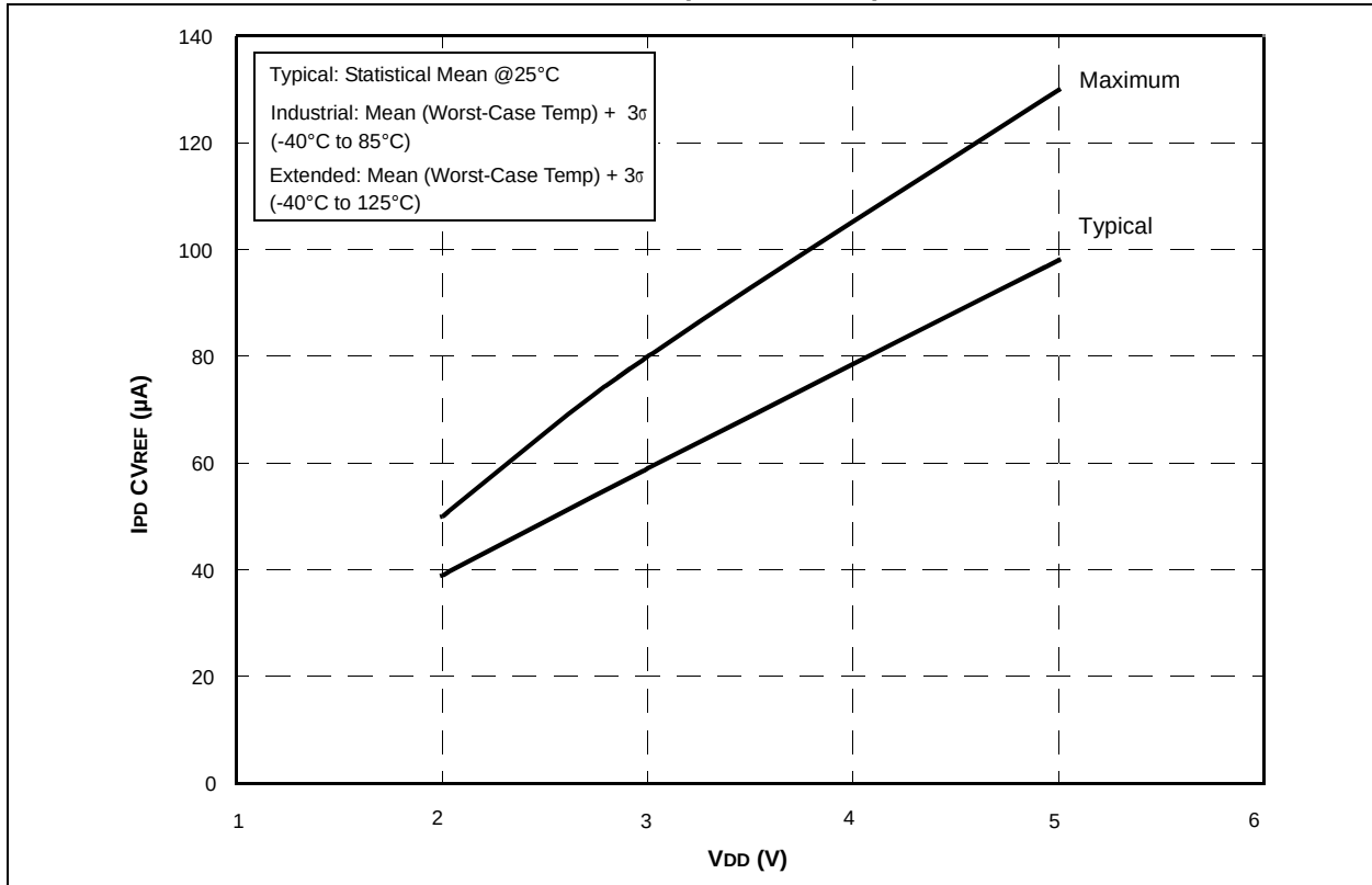
FIGURE 17-14: PIC12F609/615/617 I PD CVREF (LOW RANGE) vs. V DD
