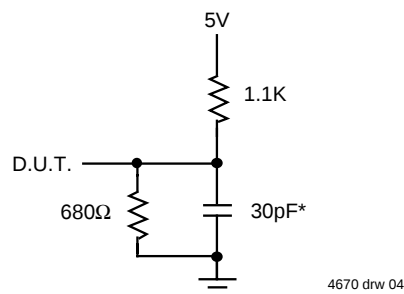
Figure 2. Output Load
