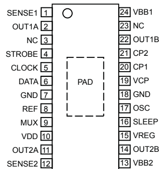
LP Package
