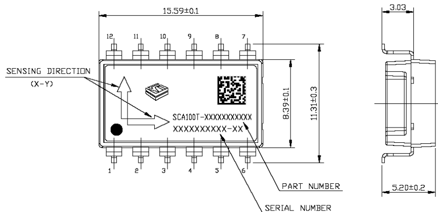
Figure 15. Mechanical dimensions of the SCA100T (Dimensions in mm)
