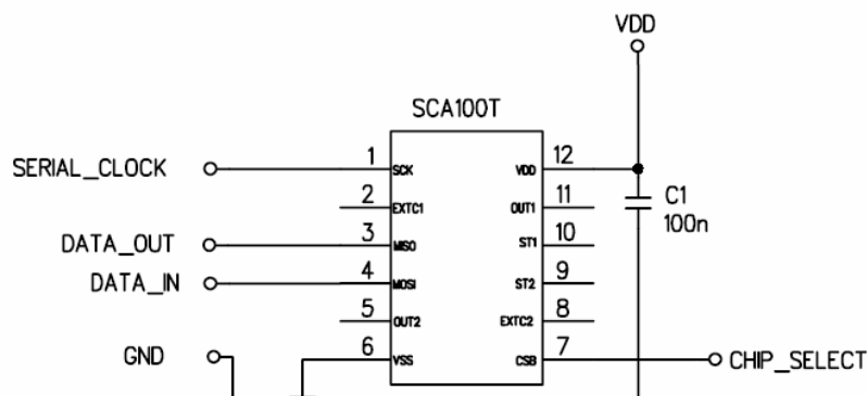
Figure 13. SPI connection example
