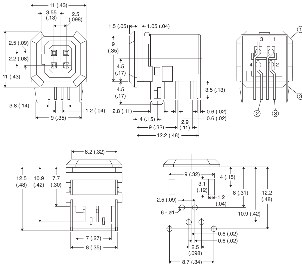
PC Board Hole Layout (Bottom View)
