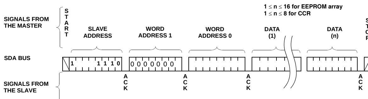
FIGURE 21. PAGE WRITE SEQUENCE
