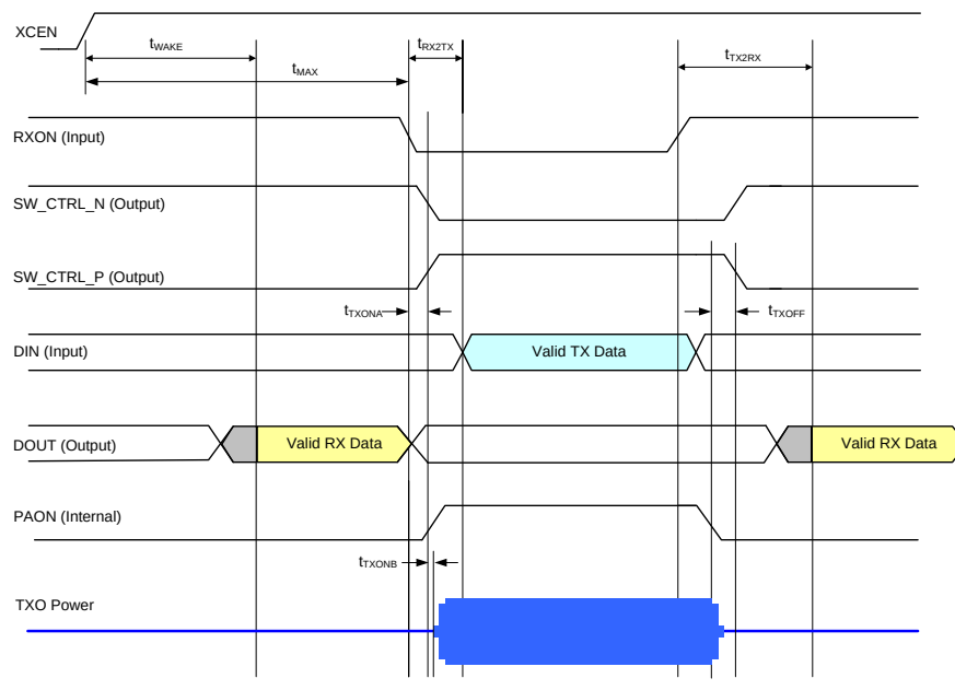
Figure 2 Control Timing for TDD Operation, PAFIRST=0 (The external switch controls SW_CTRL_P/N are switched before PA is turned on).
