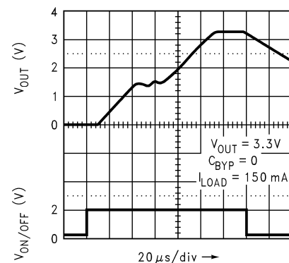
Turn-On Time
