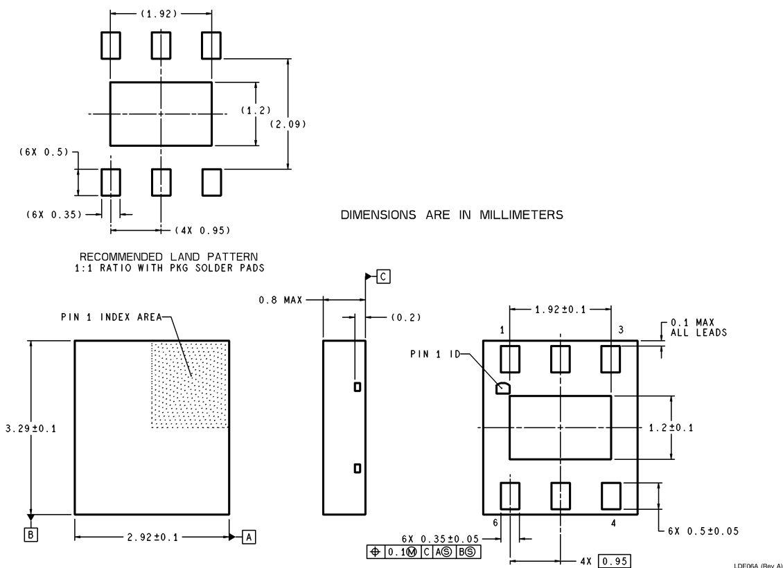
6-Lead LLP Package (LD) NS Package Number LDE06A
