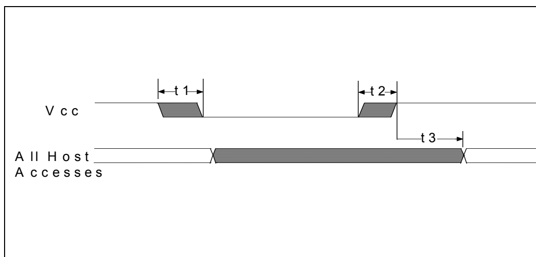
Figure 21.2 - Power-Up Timing
