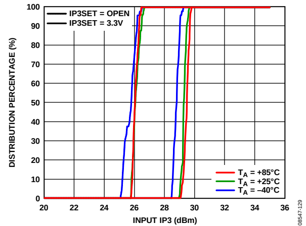
Figure 29. Input IP3
