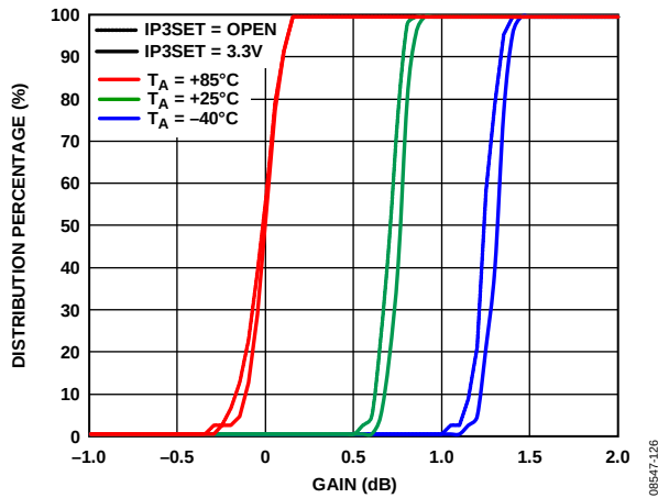
Figure 26. Gain
