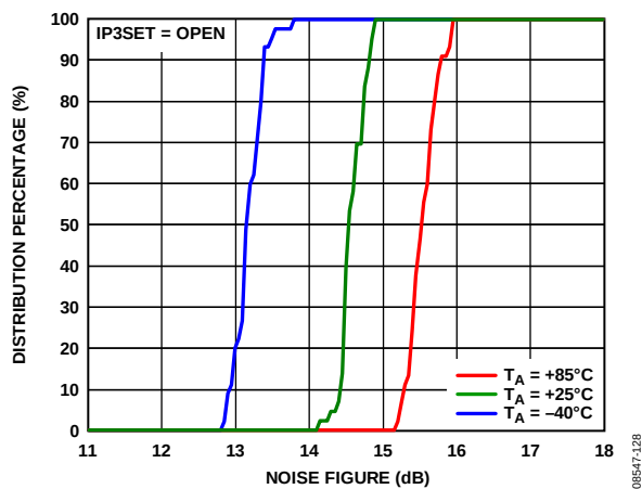
Figure 28. Noise Figure
