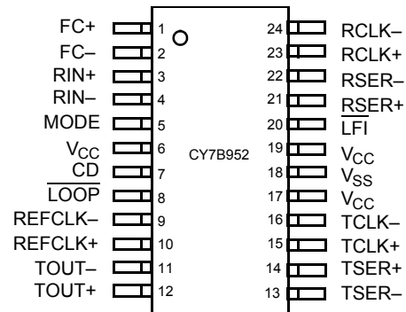
Figure 1. 24-pin SOIC (Top View)
