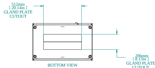
BOTTOM VIEW
