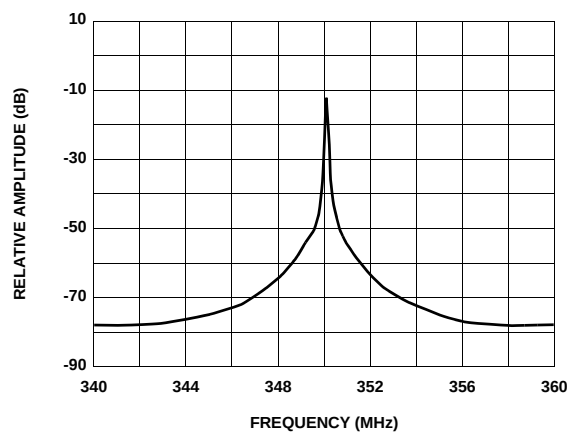
FIGURE 18. OUTPUT SPECTRUM-WIDEBAND
