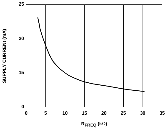
FIGURE 7. SUPPLY CURRENT vs R_{FREQ}
