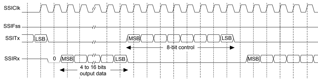
Figure 13-11. MICROWIRE Frame Format (Continuous Transfer)
