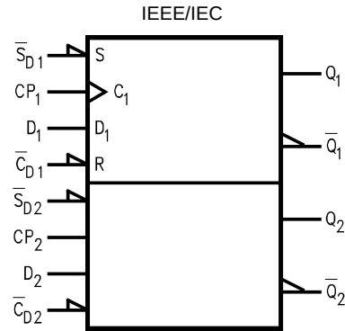
Figure 3. Logic Symbols
