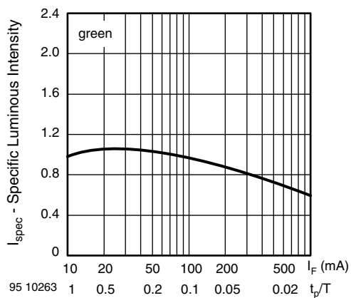
Fig. 15 - Specific Luminous Intensity vs. Forward Current
