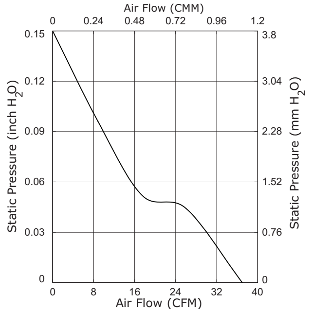
CFM-8025V-229-300
