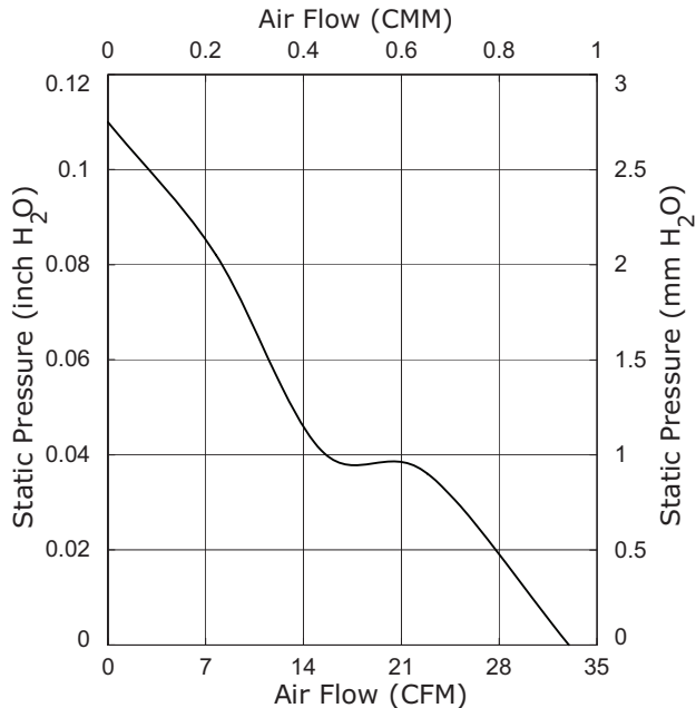
CFM-8025V-226-280
