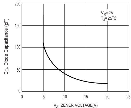
Figure2 Diode Capacitance vs. Zener Voltage
