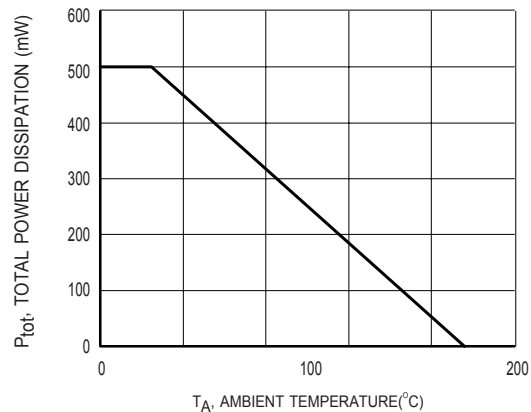
Figure1 Total Power Dissipation vs. Ambient Temperature
