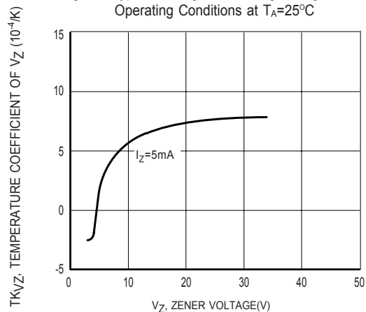
Figure5 Temperature Coefficient of V_Z vs. Zener Voltage
