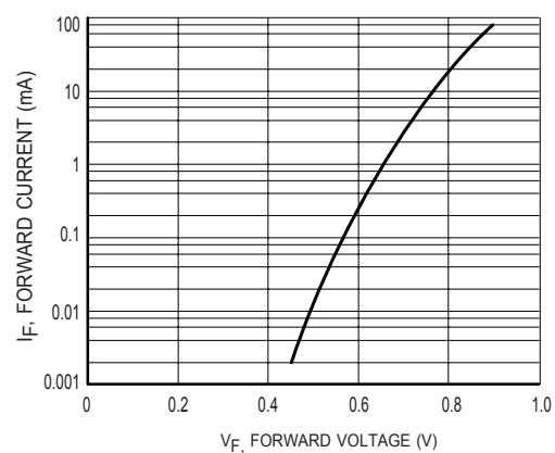
Figure6 Forward Current vs. Forward Voltage
