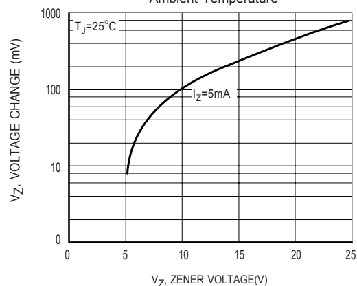
Figure3 Typical Change of Working Voltage under Operating Conditions at T_A = 25^\circ C
