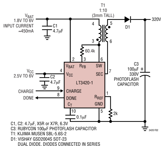
Figure 2. Small Size LT3420-1 Photoflash Circuit
