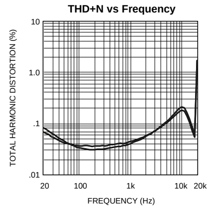
Analog V_{DD} = 2.6V , Digital V_{DD} = 2.6V R_L = 32\Omega , Power Level = 12mW R & L Channels Shown, 44.1kHz Sample Rate
