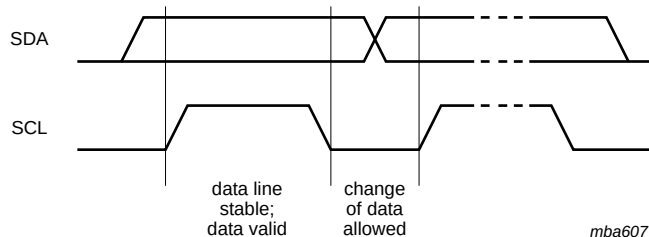
Fig 9. Bit transfer on the I 2 C-bus
