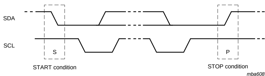
Fig 10. START and STOP conditions
