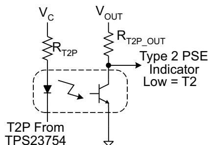
Figure 33. T2P Interface
