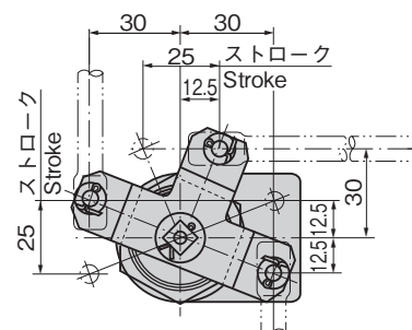
[C-310-A-1-3] [C-310-A-2-3] 3点締め Three-point securing
