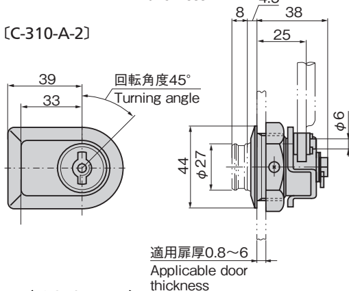
[C-310-A-1-1] [C-310-A-2-1] 1点締め One-point securing
