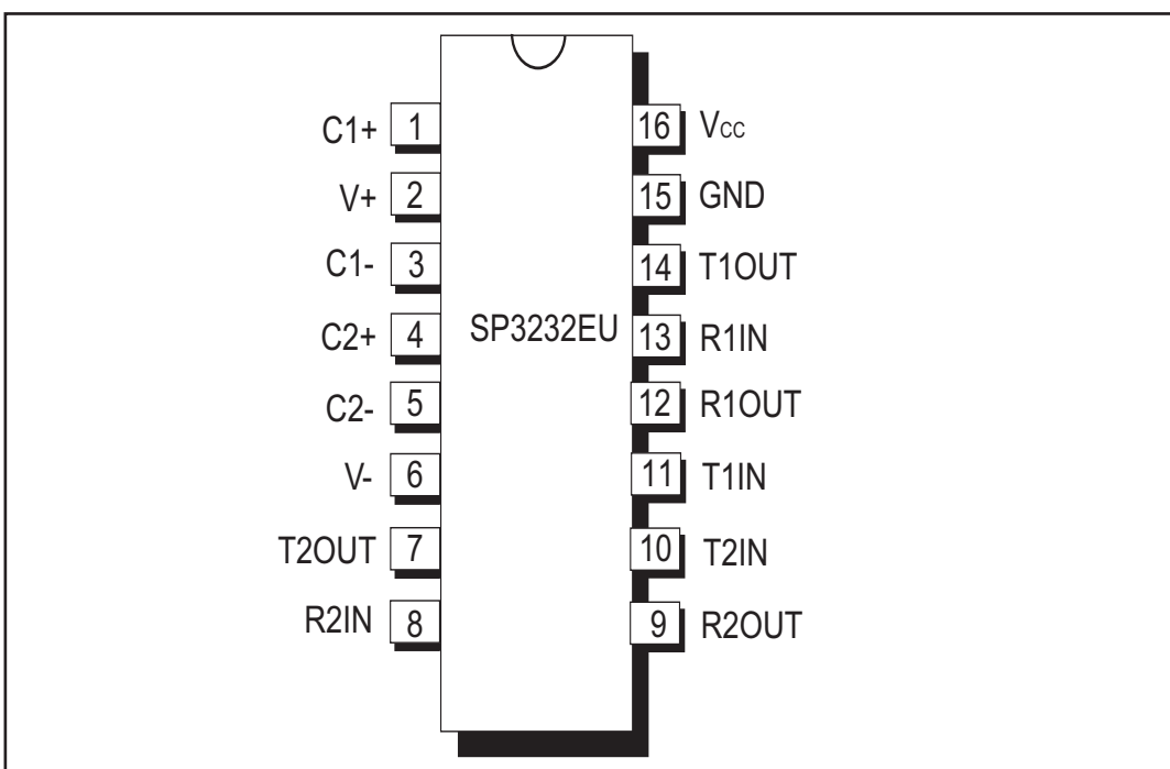
Figure 8. Pinout Configuration for the SP3232EU
