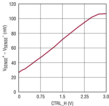
Overcurrent Threshold
