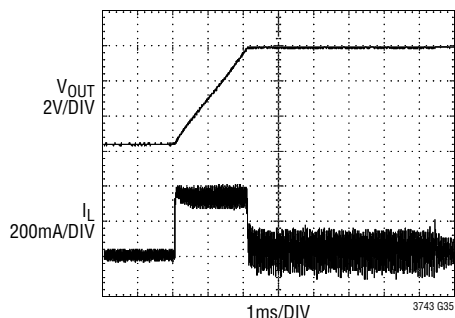
Common Mode Lockout ( V_{IN} = 7V )
