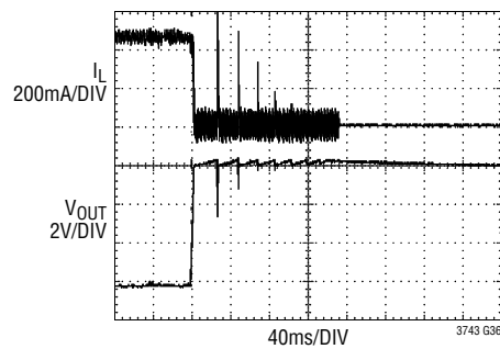
Overvoltage Lockout Operation With Open-Load Condition
