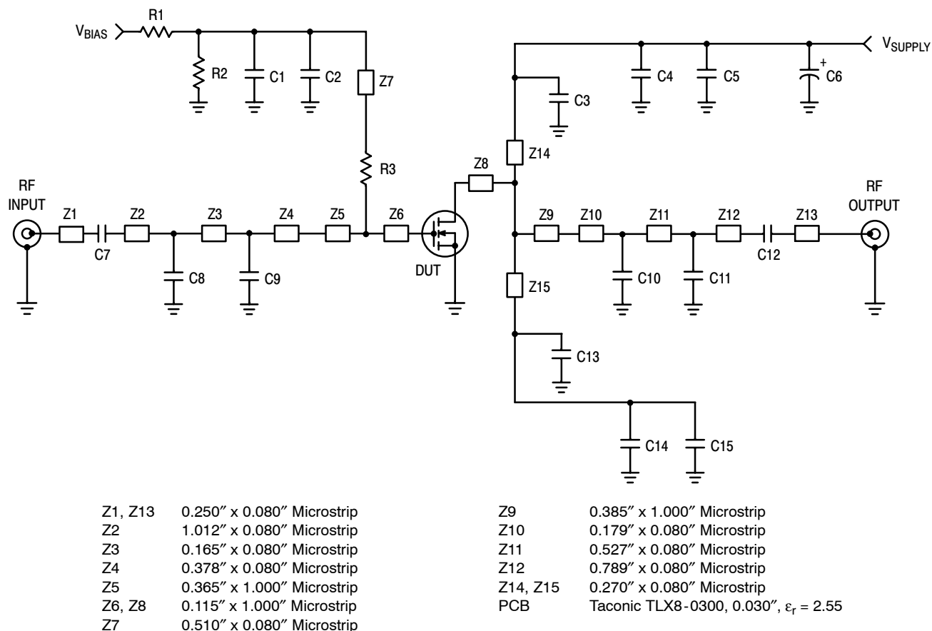
Figure 2. MRF5P21045NR1 Test Circuit Schematic — Single-Ended Configuration
