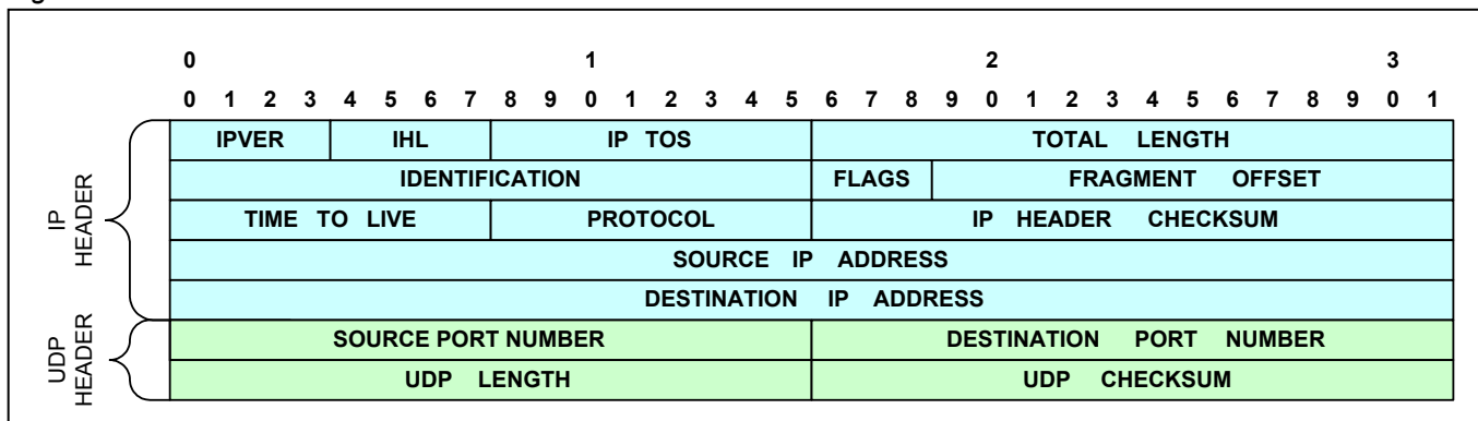
Figure 10-13. UDP/IPv4 Header Format
