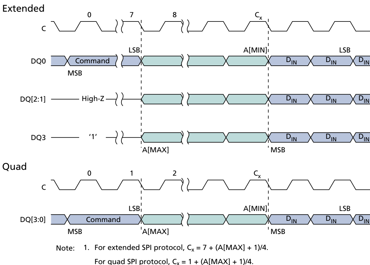
Figure 25: EXTENDED QUAD INPUT FAST PROGRAM Command
