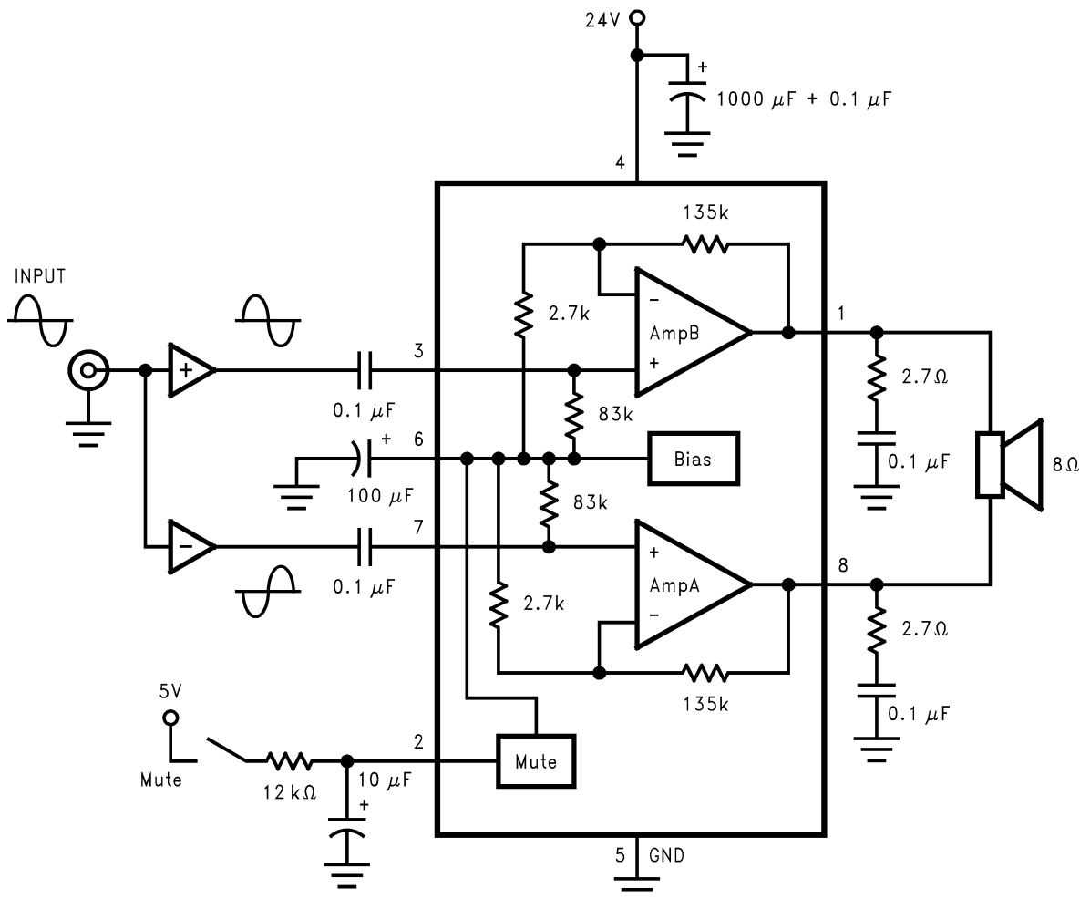
Figure 43. Bridge-Mode Application
