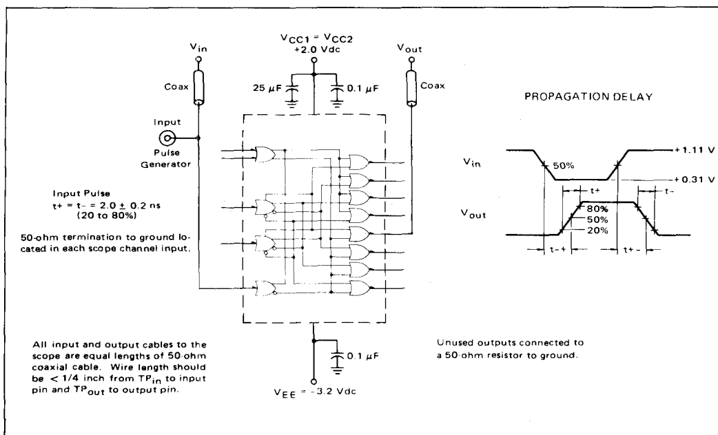
SWITCHING TIME TEST CIRCUIT AND WAVEFORMS @ 25°C
