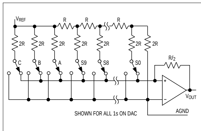
Figure 1. D/A Simplified Circuit Diagram
