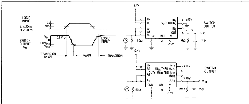
Figure 2. Transition Time Test Circuits
