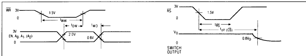
Figure 1. Typical Timing Diagrams for MAX368/369
