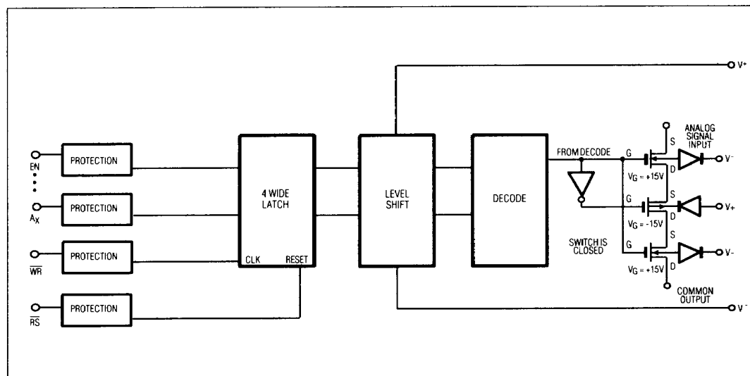
Figure 12. Simplified Internal Structure
