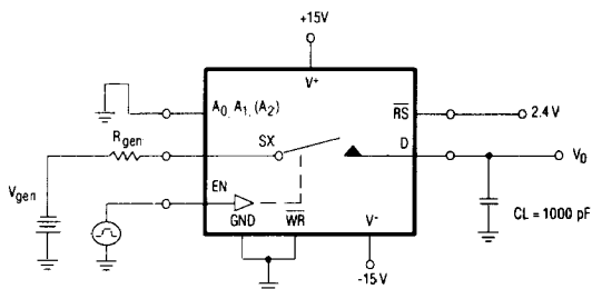
Figure 6. Reset Turn-Off Time t_{OFF}(\overline{RS}) Test Circuit
