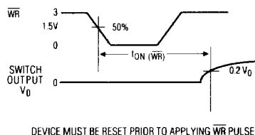
Figure 5. Write Turn-On Time t_{ON}(\overline{WR}) Test Circuit
