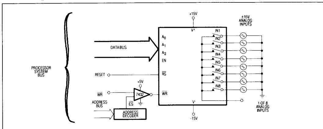
Figure 13. Bus Interface
