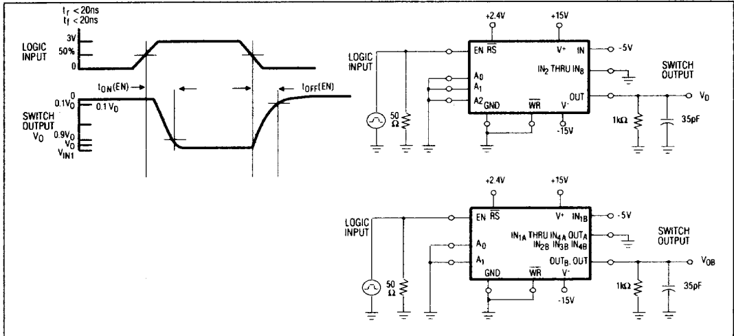
Figure 3. Enable t_{ON}/t_{OFF} Time Test Circuit
