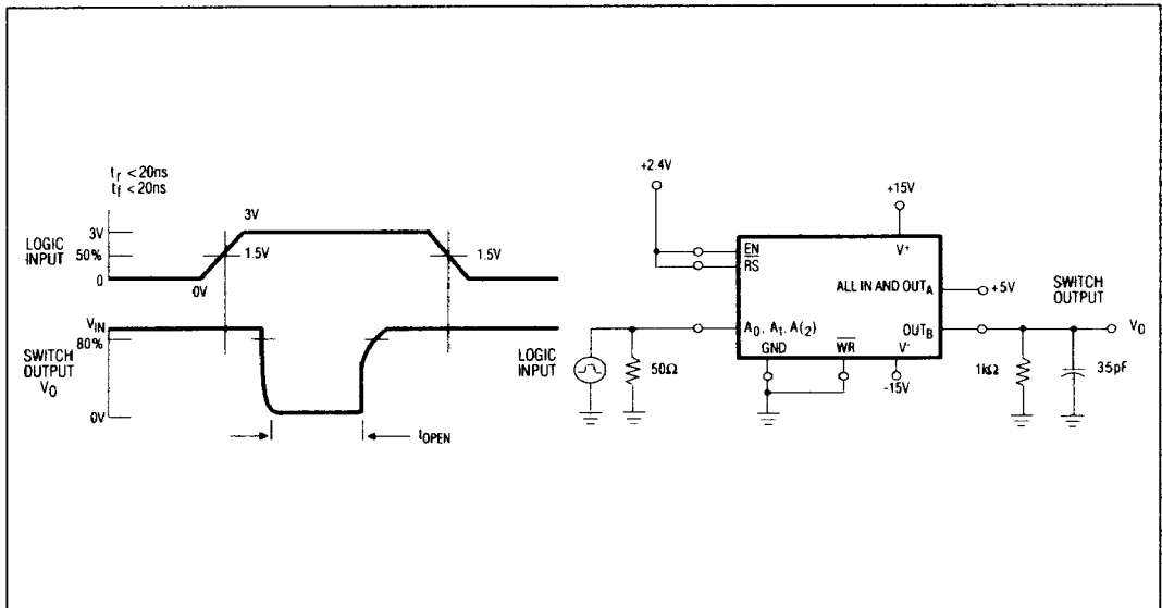
Figure 4. Open Time (B.B.M.) Interval Test Circuit
