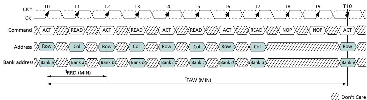
Figure 44: Multibank Activate Restriction
