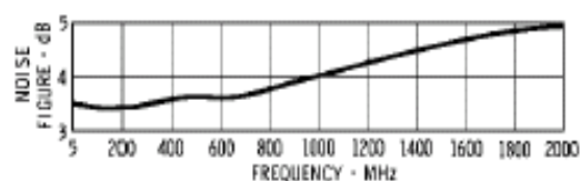
Noise Figure
