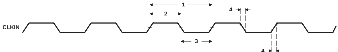
Figure 31. CLKIN Timings
