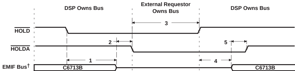
Figure 47. \overline{\text{HOLD}}/\overline{\text{HOLDA}} Timing
