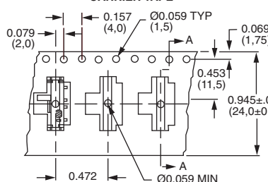
CARRIER TAPE
