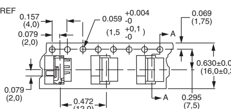
CARRIER TAPE
