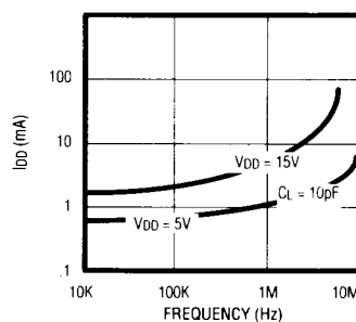
NO LOAD I_{DD} VS. FREQUENCY
