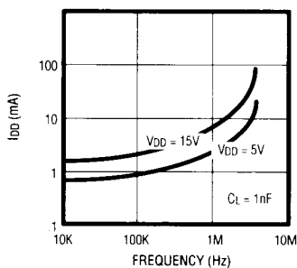
I_{DD} VS. FREQUENCY
