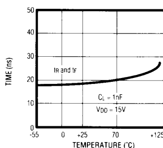
RISE AND FALL TIMES VS. TEMPERATURE
