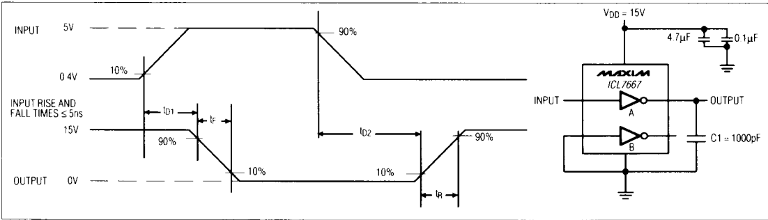
Figure 1. Test Circuit
