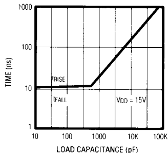
RISE AND FALL TIMES VS. C_L
