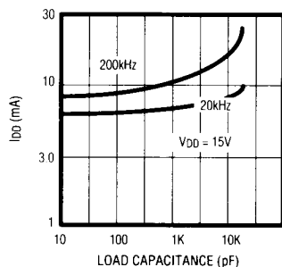
I_{DD} VS. C_L
